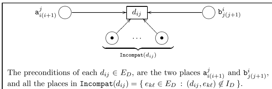
Figure 6.2: The elementary net system N(T) .
