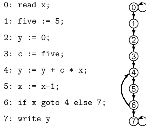
Figure 1. Example program and control flow graph.
