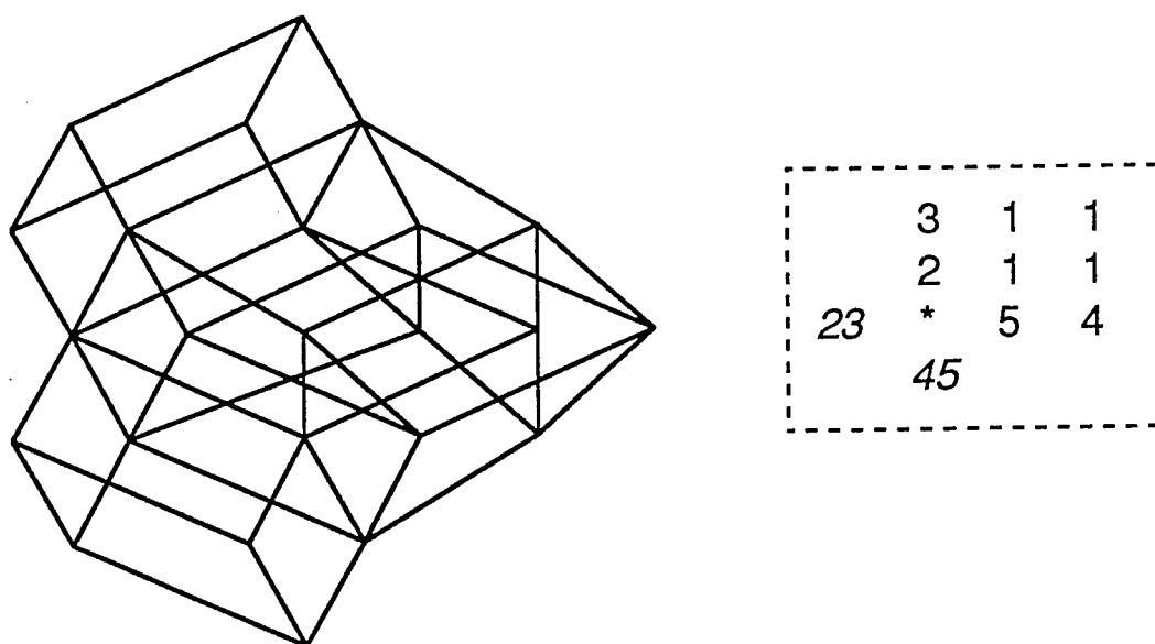
Figure 11: A lattice interval in FDL(5) and its associated configuration
