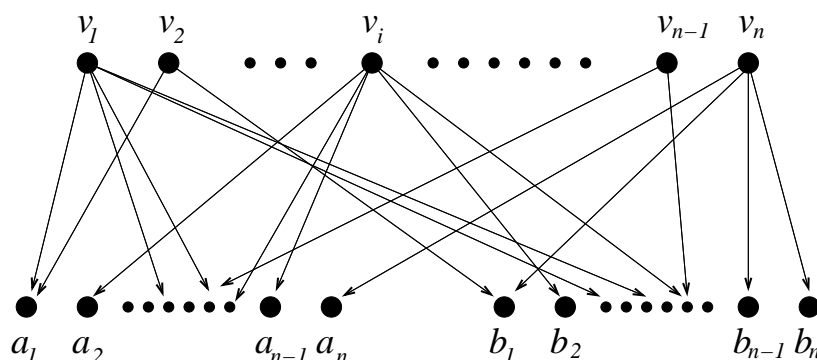
Figure 2: A scheme of the construction used in the proof of Theorem 12.
