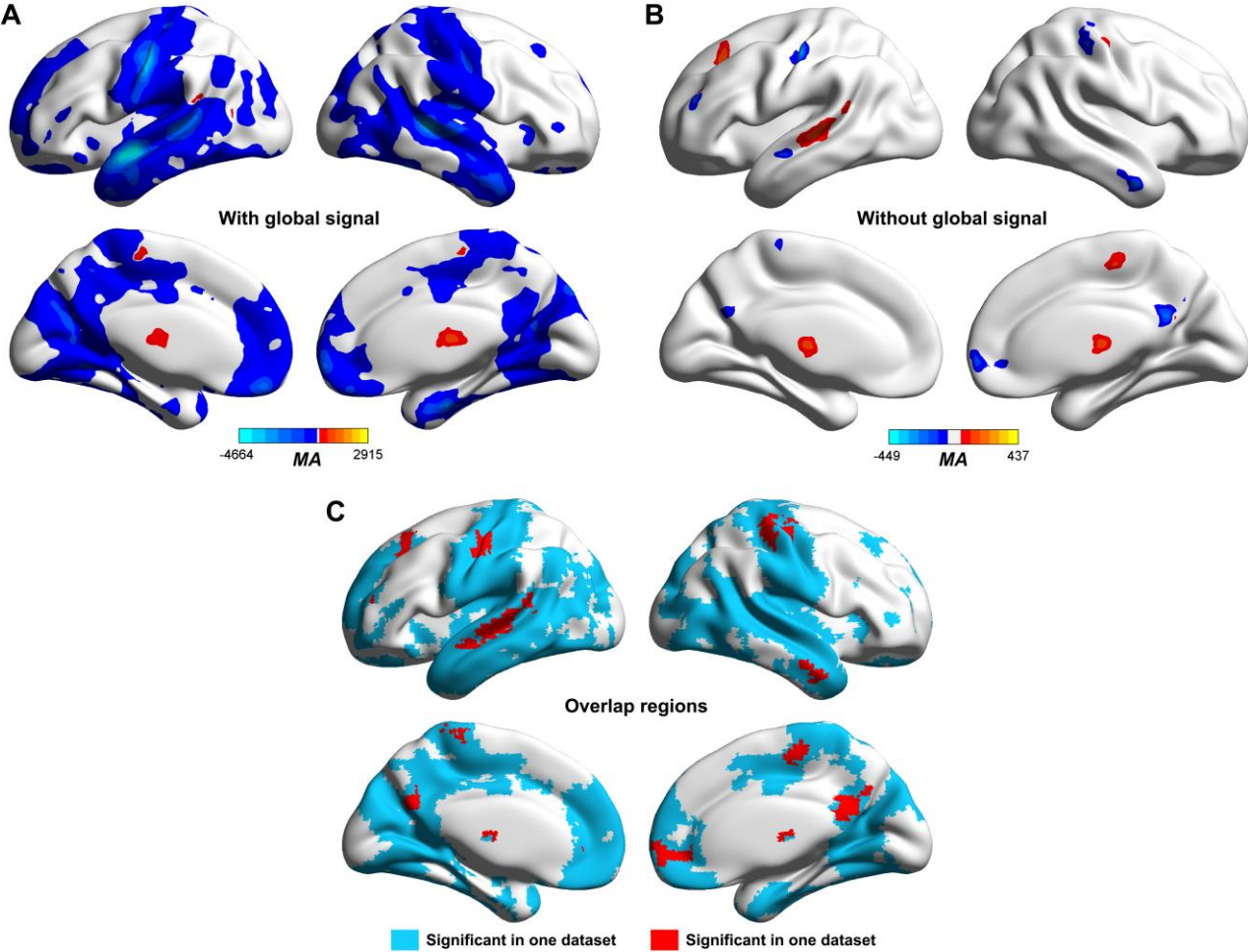
Figure S6. Comparison between the result with (A) and without (B) global signal.
