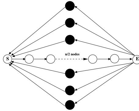
Figure 3: A good graph for the rabbit
