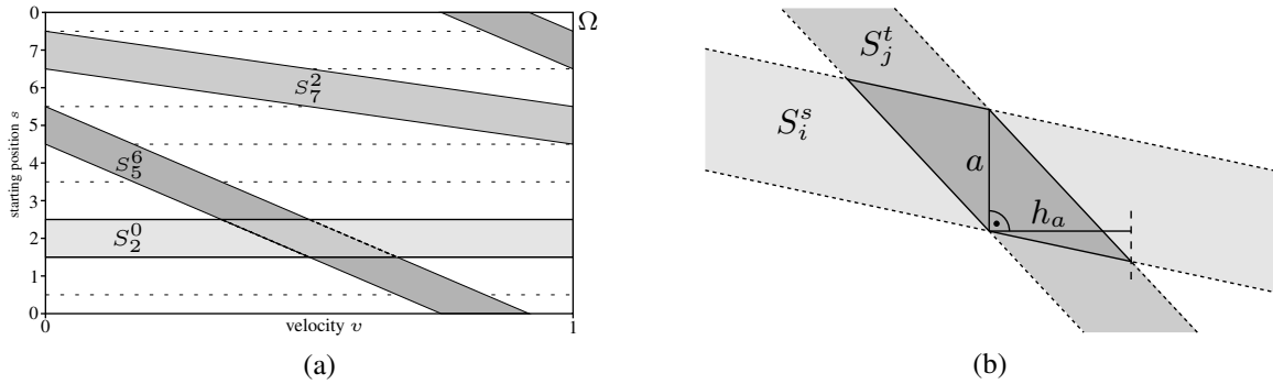
Figure 1: (a) The sample space \Omega of the RANDOMSPEED strategy can be viewed as the surface of a cylinder. The sets S_i^t correspond to stripes on this surface. (b) The intersection between two stripes of slope -s and -t , respectively.
