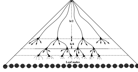
Figure 2: Embedding of the recursion tree T_S into the tree T .
