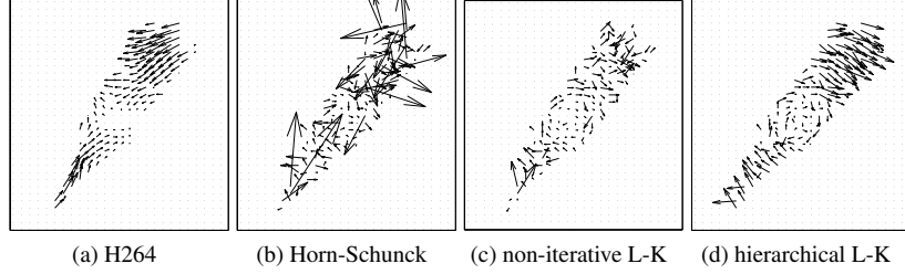
Figure 2: Optical flows for synthetic sequence, frame 1.
