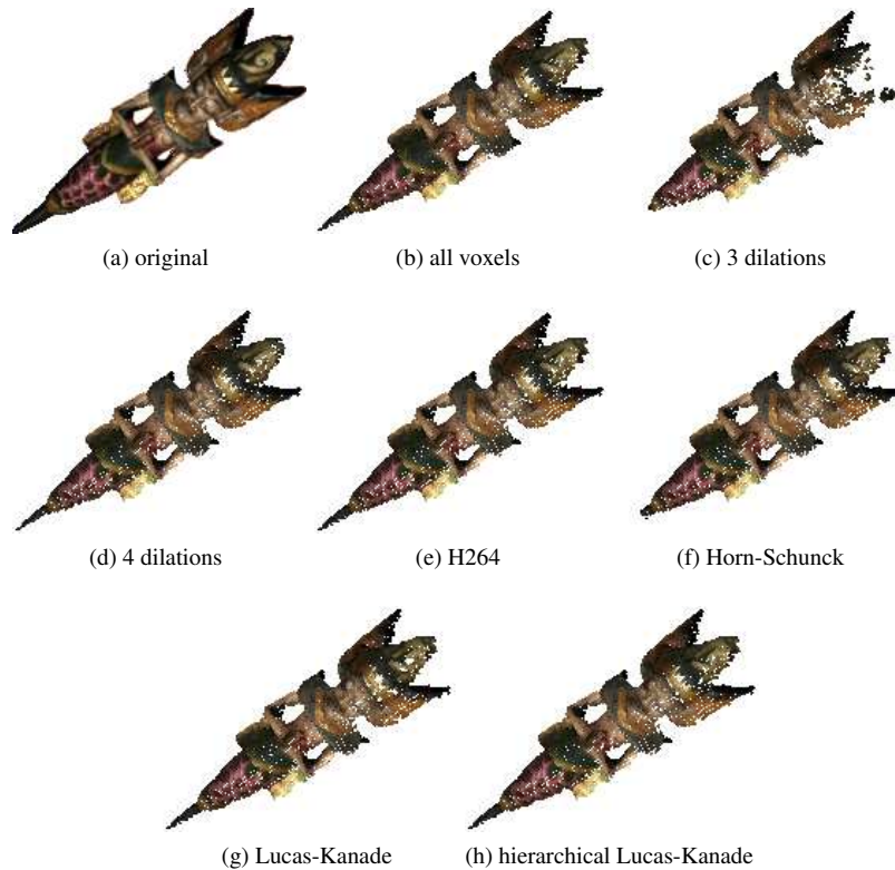
Figure 6: Frame 19 reconstructions for synthetic sequence.
