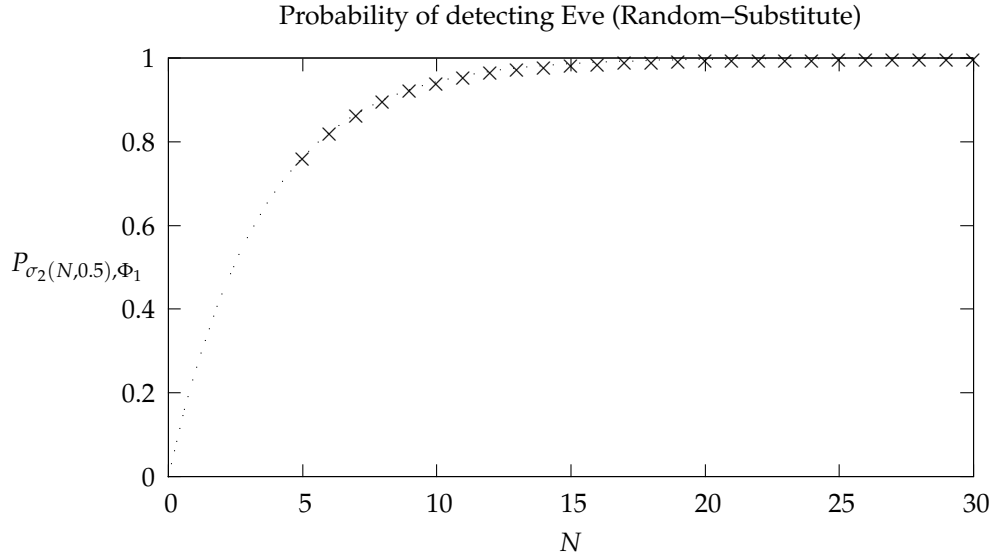
Figure 4.2 The probability that Eve is detected in the BB84 Protocol while performing a random-substitute attack, as a function of the security parameter N .
