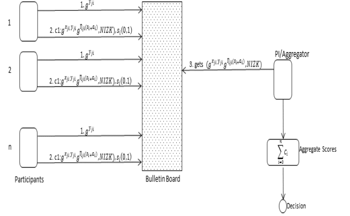
Fig. 2: Workflow of privy System.
