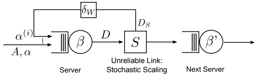
Figure 1. Network calculus model of an unreliable link with retransmissions.
