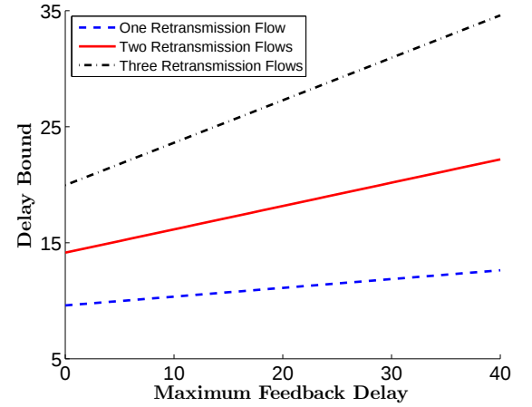
Figure 6. Delay bounds with changing maximum feedback delay (loss probability p = 0.7 ).
