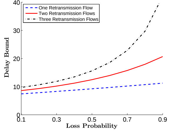
Figure 5. Delay bounds with retransmission attempts i ( i = 1, 2, 3 ).
