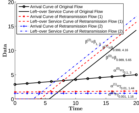
Figure 4. Arrival, service curves, and delay bounds.
