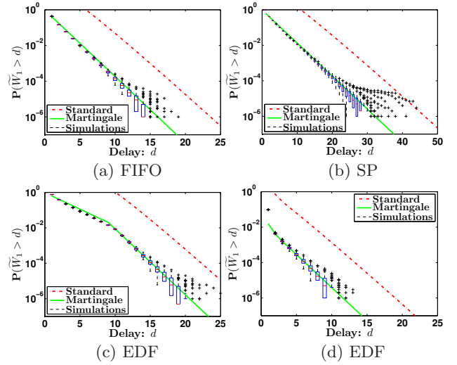
Figure 1: Delay bounds ( \lambda = 0.5 , \mu = 0.1 , P = 1 , n_1 = n_2 = 10 , \rho = 75\% , ( d_1^* = 10 , d_2^* = 1 ) in (c) and d_1^* = 1 , d_2^* = 10 in (d))
