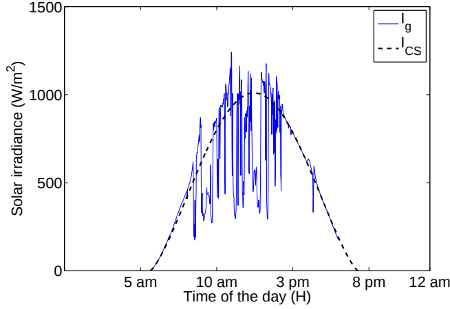
Fig. 2: Illustrating the global and the clear sky irradiance for a sample day.
