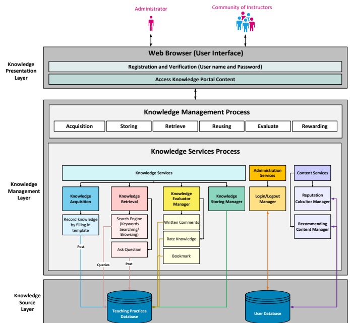
Fig. 5. TPMS Architecture
