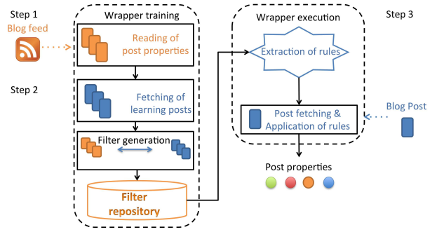
Figure 1: Overview of the weblog data extraction approach.
