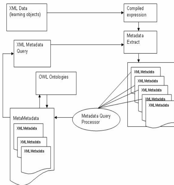
Fig. 3 The OMESCOD architecture work flows
