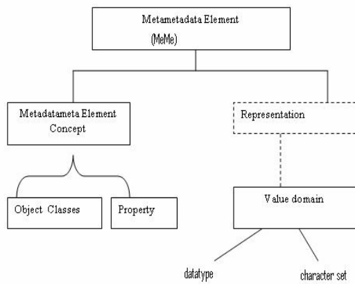
Fig. 1 Metametadata Element Concept
