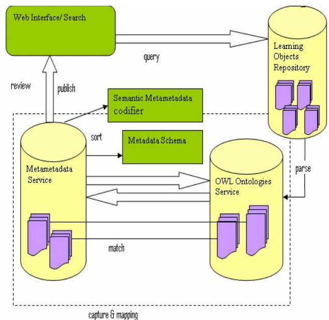
Fig. 4 OMESCOD Architecture
