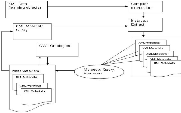
Fig. 5: The OMESCOD architecture and Metametadata development
