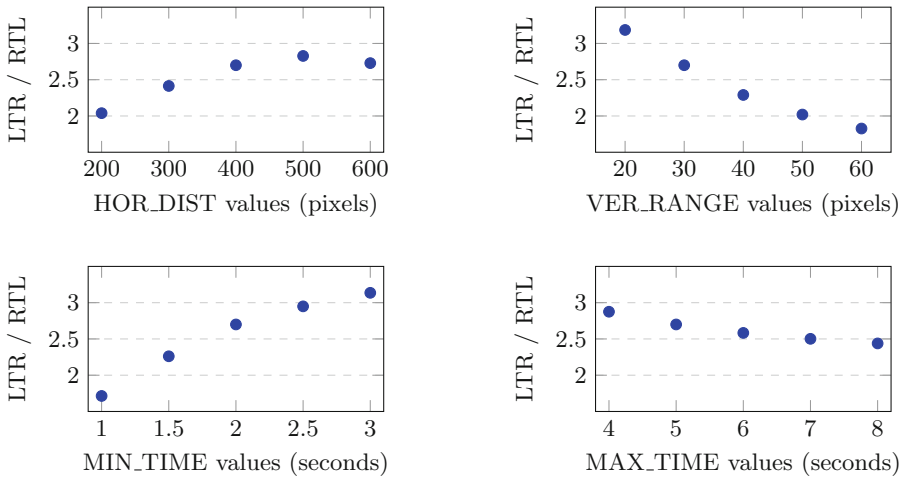
Fig. 2. LTR HMMs/RTL HMMs ratio with different parameters
