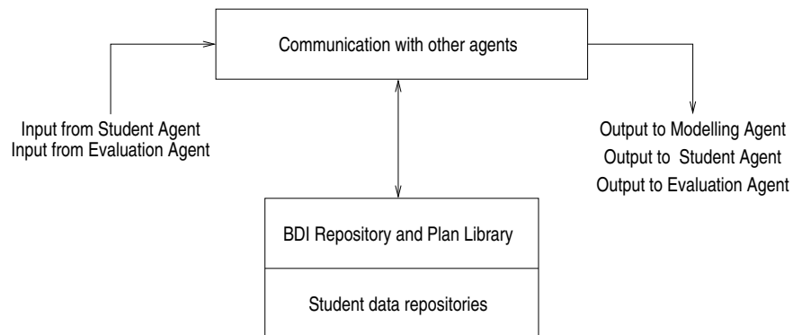
Figure 3: Record Agent.
