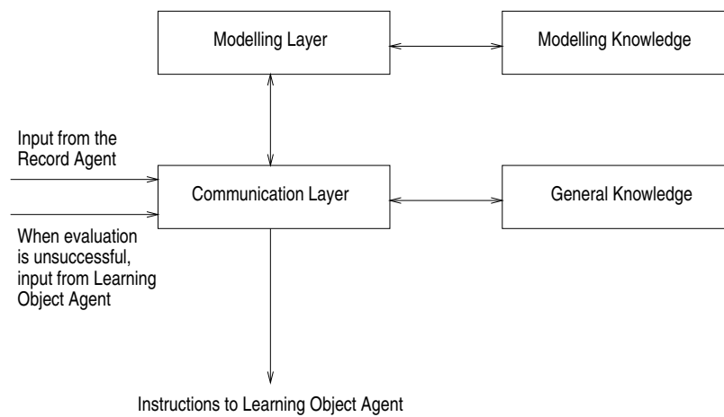
Figure 4: Modelling Agent.
