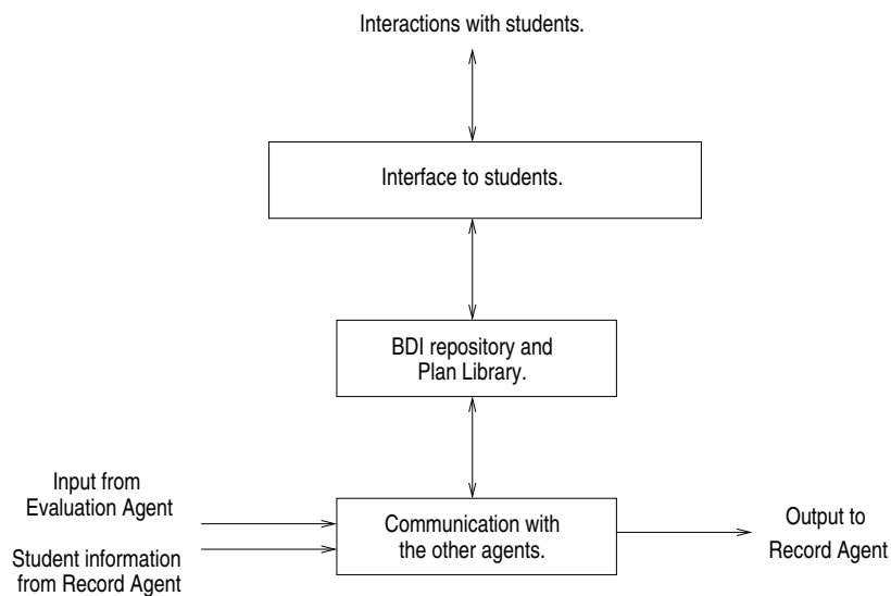
Figure 2: Student Agent.
