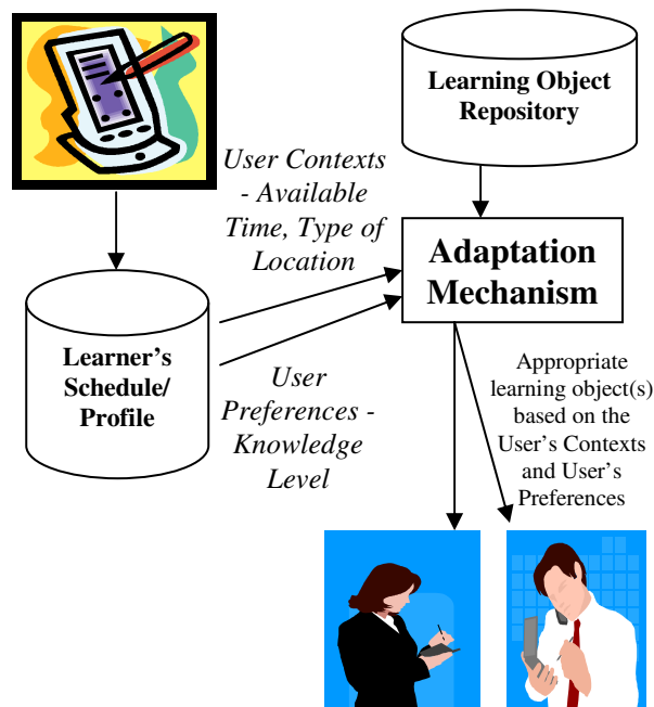
Figure 1 – Conceptual Model of mCALS
